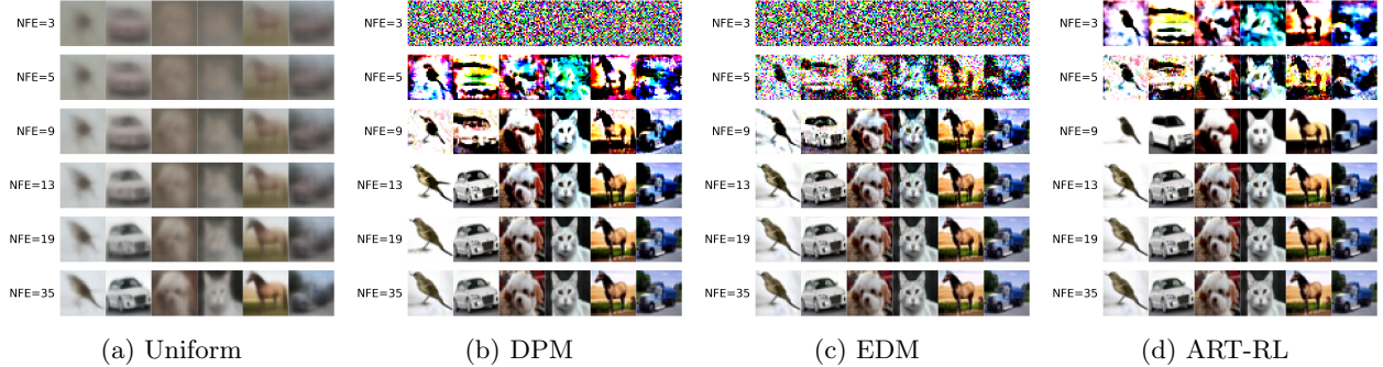
Figure 6: CIFAR-10 samples across timesteps for the four schedules (Uniform, DPM, EDM, ART-RL). Each panel shows a 6 \times 6 grid where rows correspond to increasing NFE.
