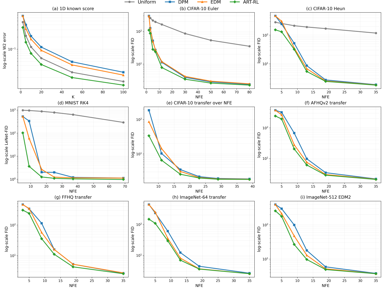
Figure 3: Visual overview of ART-RL across experiments. Each panel uses a logarithmic vertical axis and compares schedules at matched timestep counts or matched NFE. DPM denotes the DPM-Solver timestep grid.
